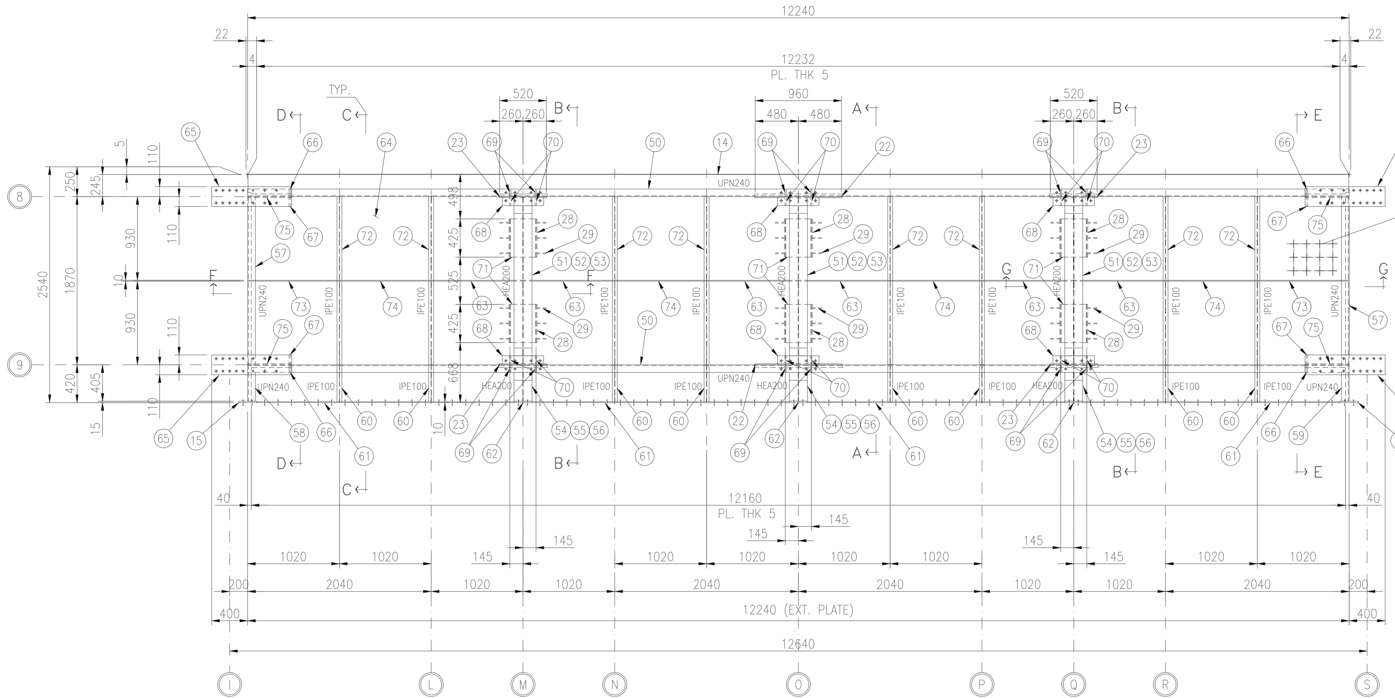
FLOOR PLAN CONVECTION E-020 1:25 VIEW FROM BELOW E020-B
